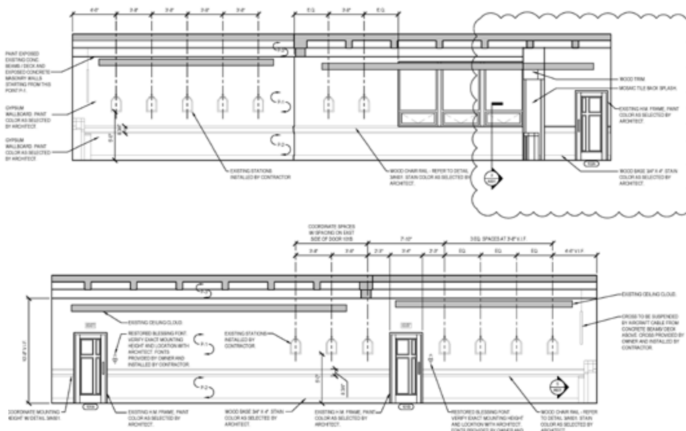
Developed Interior Elevations
