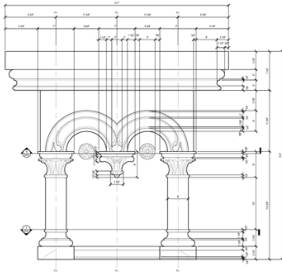
Dimensioned Altar Elevation
